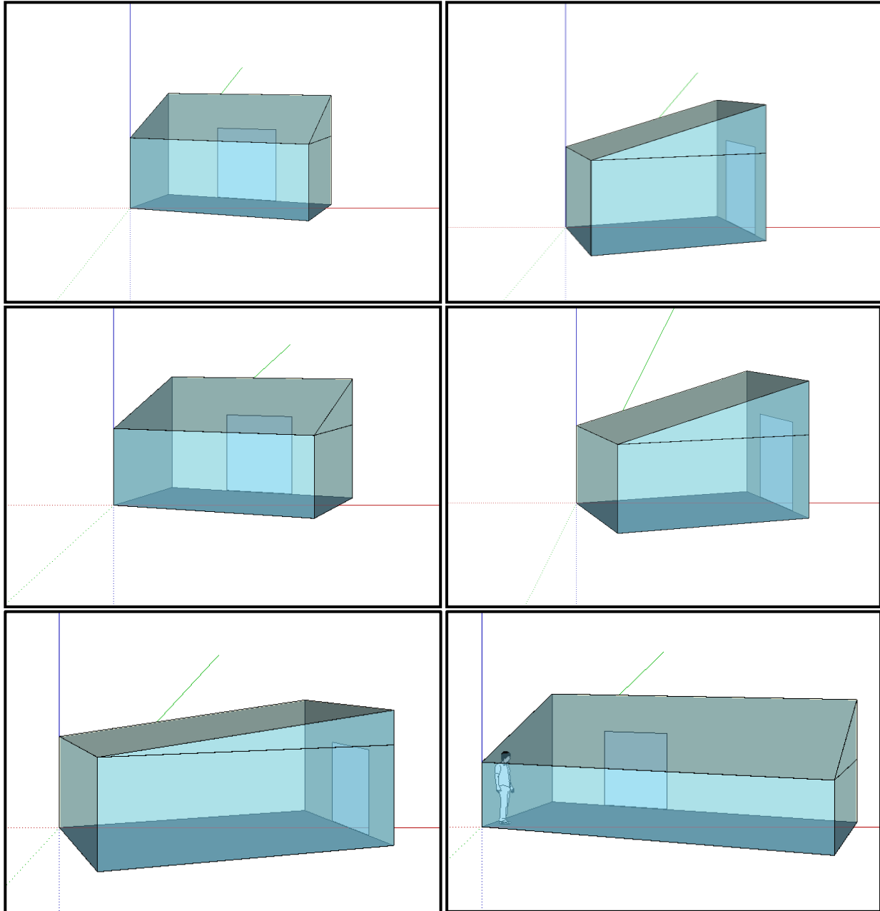
Image 1: Solarium designs – floor area and orientation – 12m 2 20°W (upper left), 12m 2 70°W (upper right), 15m 2 20°W (centre left), 15m 2 70°W (centre right), 30m 2 20°W (lower left) 30m 2 , 70°W (lower right) (green axis is due north)
