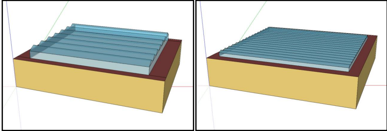
Image 2: Rooftop greenhouse designs – 1,400 m 2 , 20°W (left) - 7,000 m 2 , 20°W (right)
